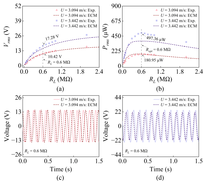
Fig. 9. Experimentally measured and ECM simulated outputs of the VGPEH with the 40-0.5 bluff body connected to an ac circuit. (a) RMS voltage outputs V_{rms} versus the load resistance. (b) RMS output power outputs P_{rms} versus the load resistance. (c) Steady-state time-history voltage responses at R_L = 0.6 M \Omega and U = 3.094 m/s. (d) Steady-state time-history voltage response at R_L = 0.6 M \Omega and U = 3.442 m/s.
